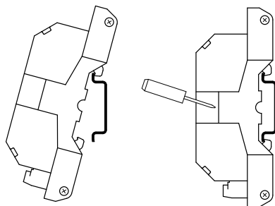
Fig. 1: Installation
